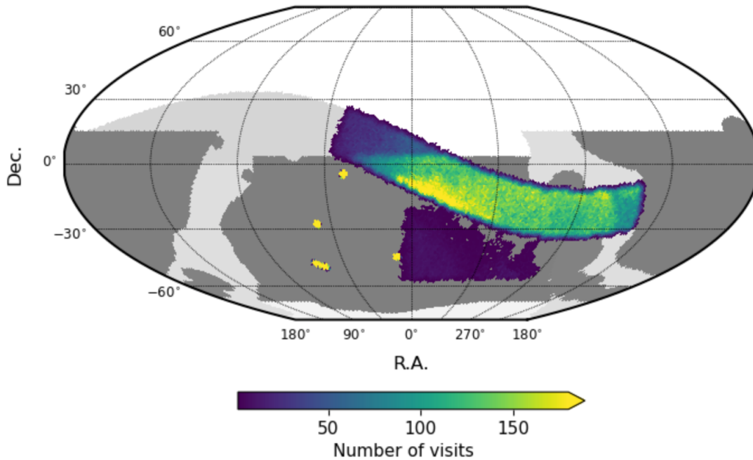
FIGURE 4: SV surveys coverage expressed as total number of overlapping visits across the ugrizy bands.
